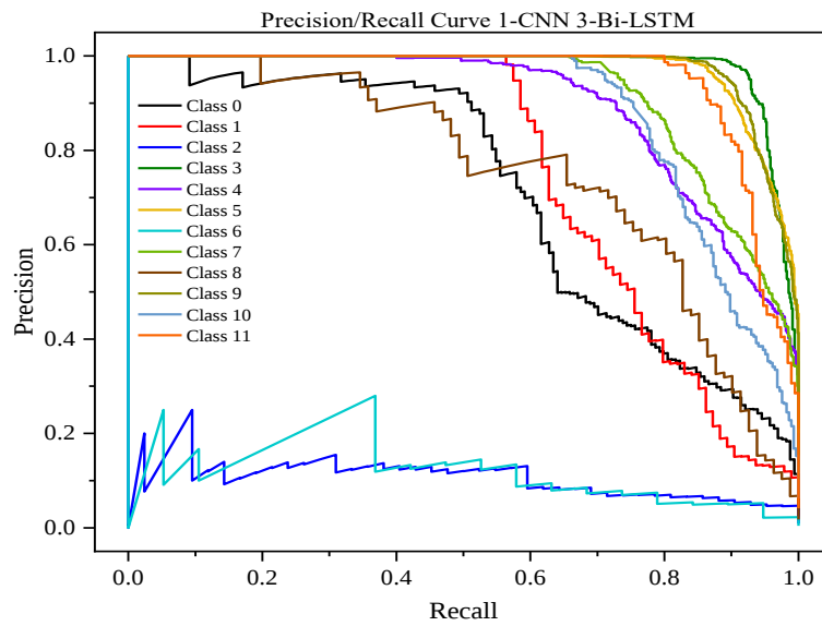
Figure 8: The precision/recall curve 1-CNN 3-Bi-LSTM of every class
