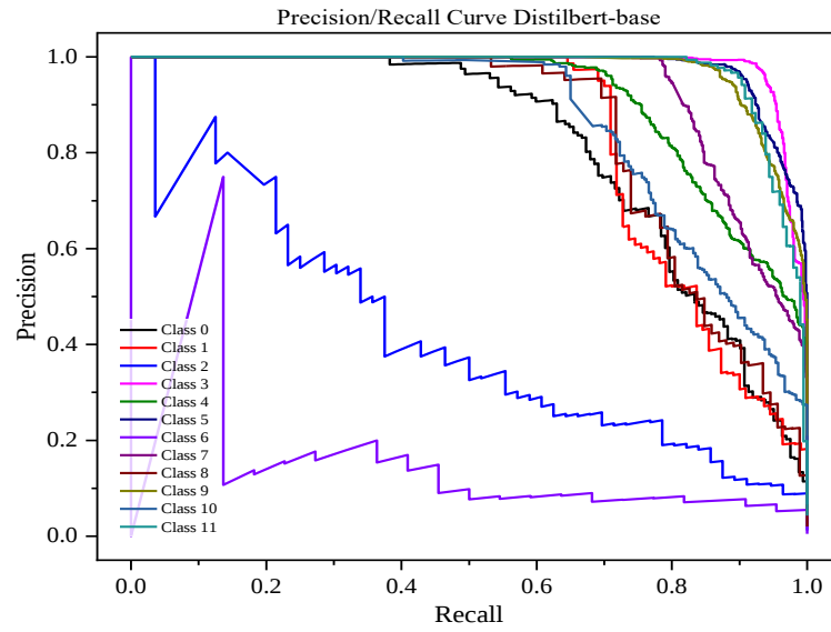
Figure 7: The precision/recall curve is distilbert-base-uncased for every class
