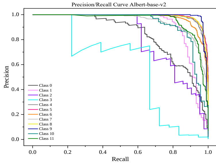
Figure 11: The precision/recall curve Albert-base-v2 of every class
