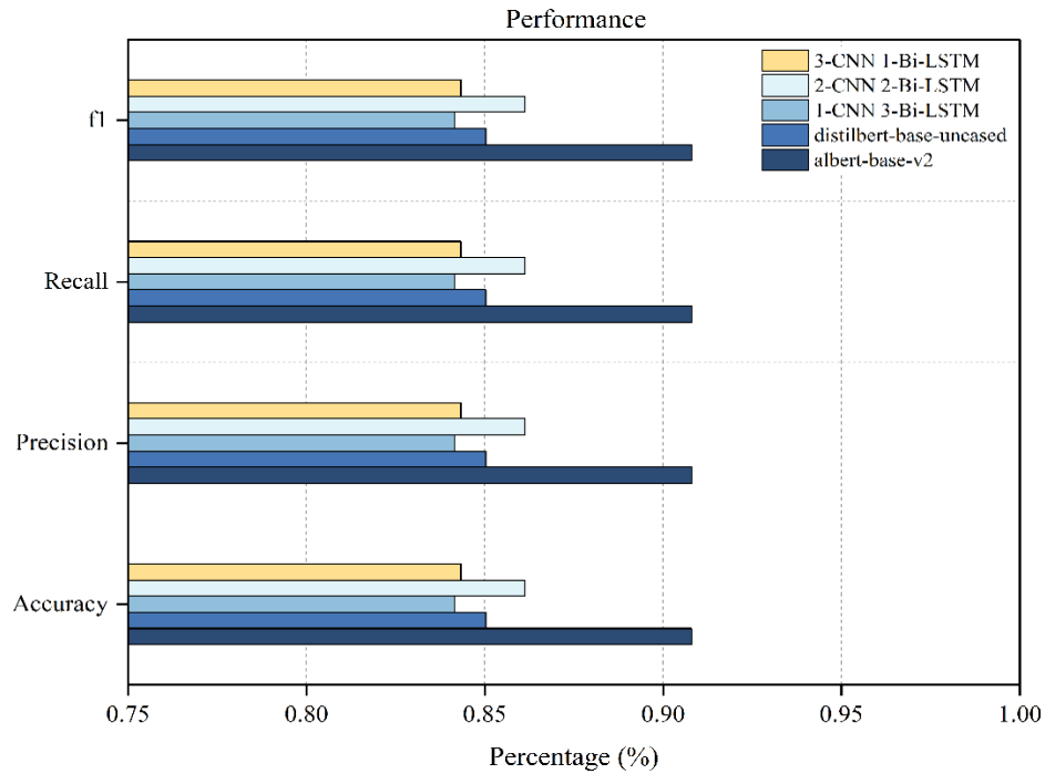
Figure 14: The performance obtained from albert-base-v2, 2-CNN 2-Bi-LSTM, disitilbert-base-uncased, 3-CNN 1-Bi-LSTM, and 1-CNN 3-Bi-LSTM classification models
