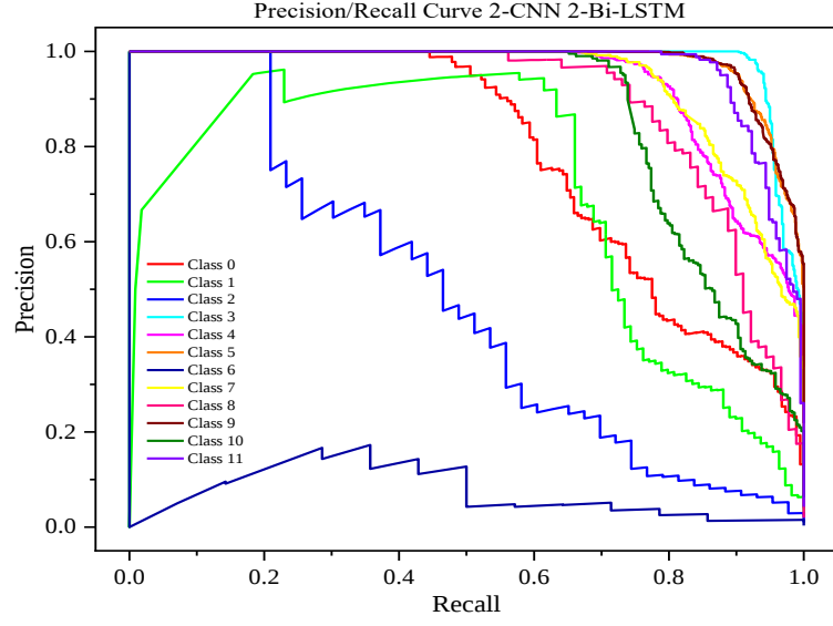
Figure 9: The precision/recall curve 2-CNN 2-Bi-LSTM of every class
