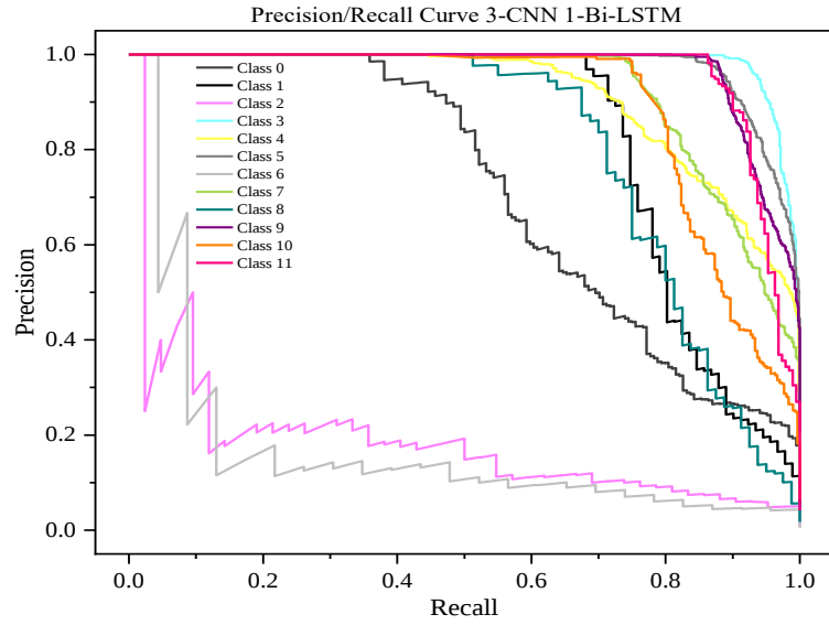
Figure 10: The precision/recall curve 3-CNN 1-Bi-LSTM of every class
